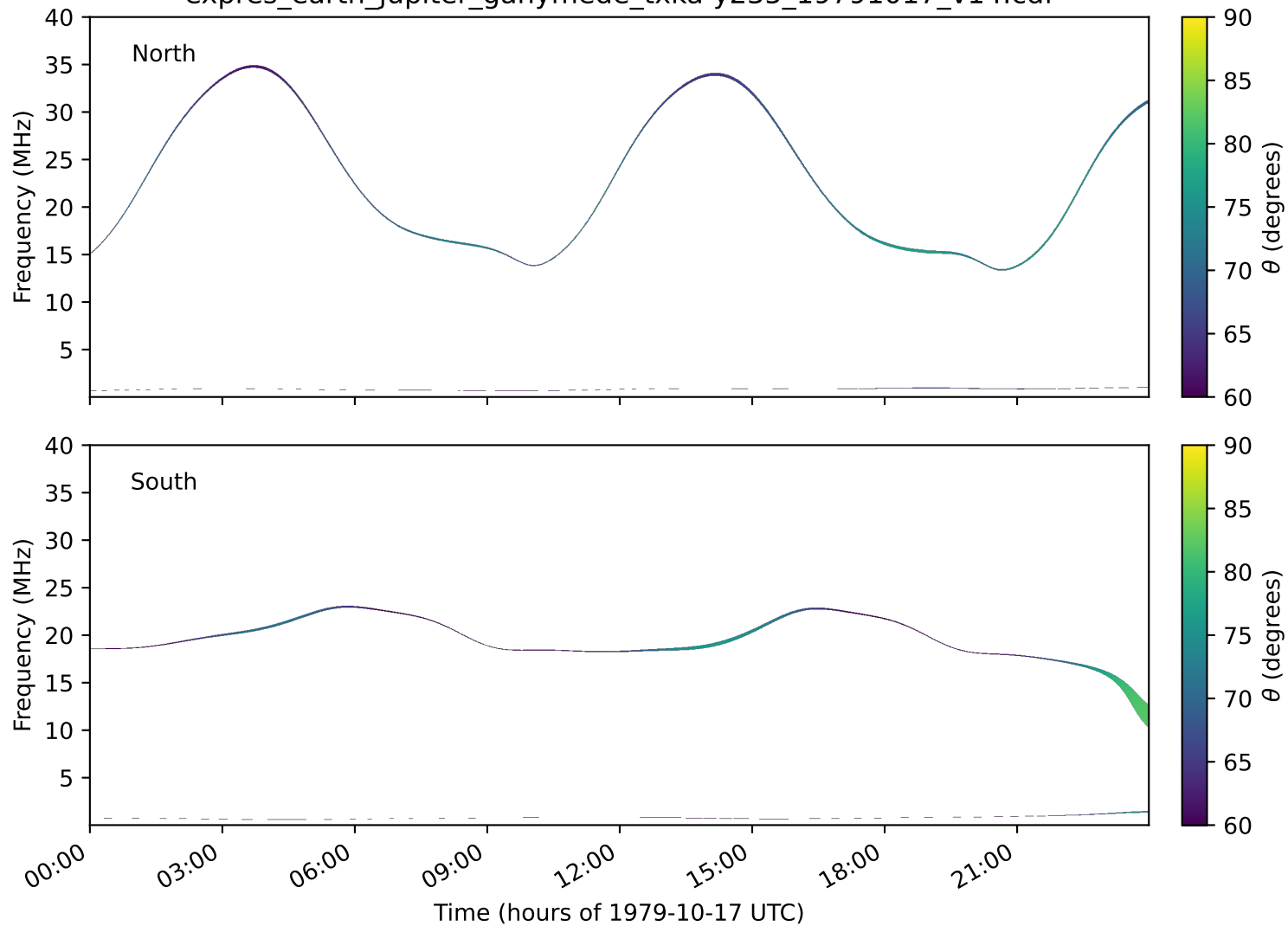
expres_earth_jupiter_ganymede_txka-y235_19791017_v14.cdf
