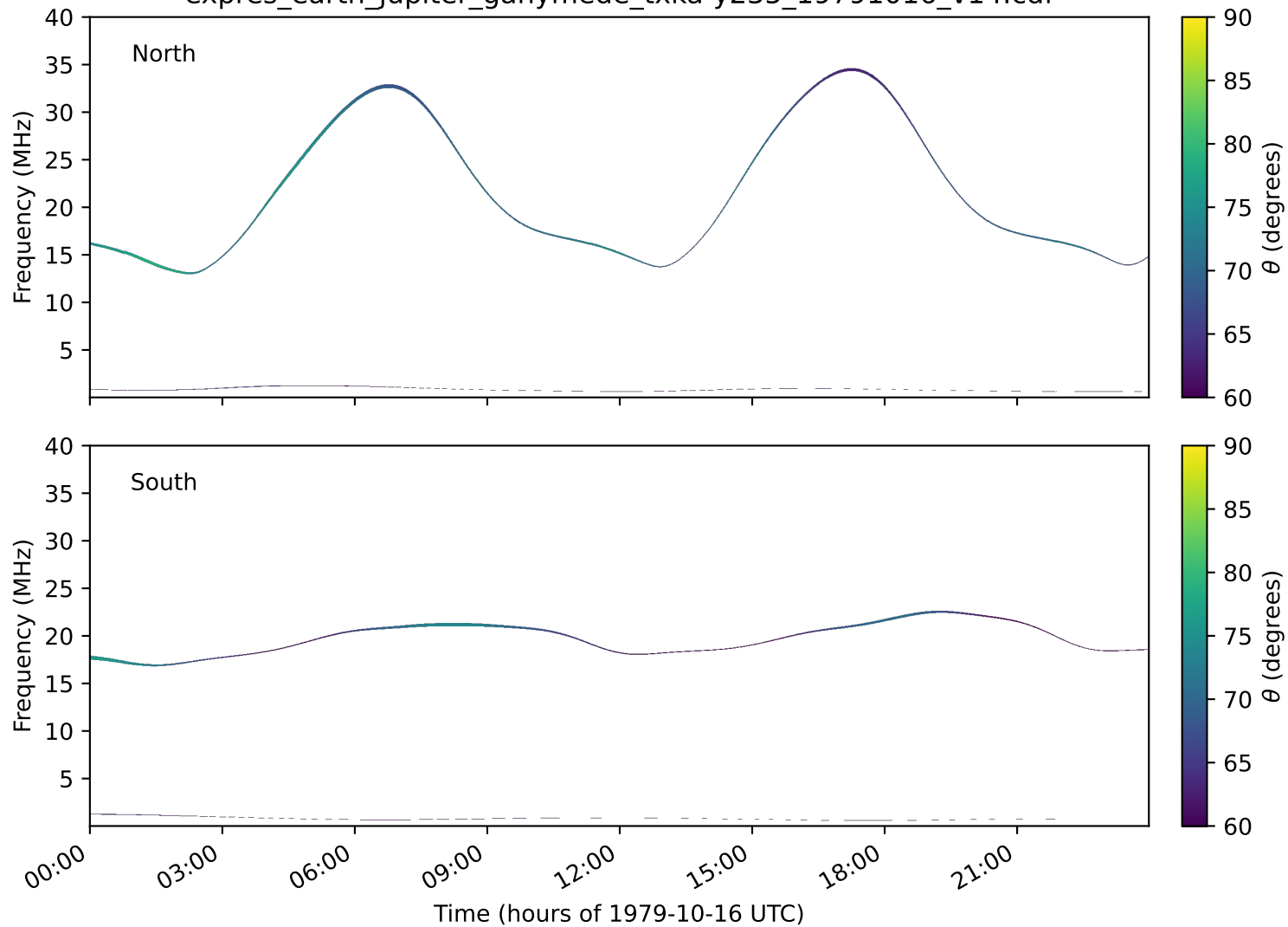
expres_earth_jupiter_ganymede_txka-y235_19791016_v14.cdf
