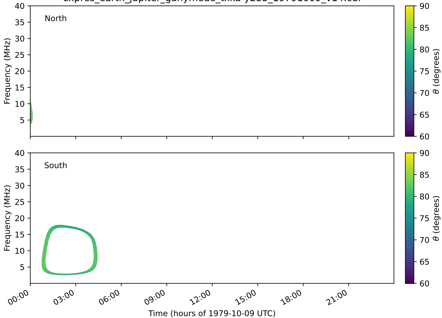
expres_earth_jupiter_ganymede_txka-y235_19791009_v14.cdf
