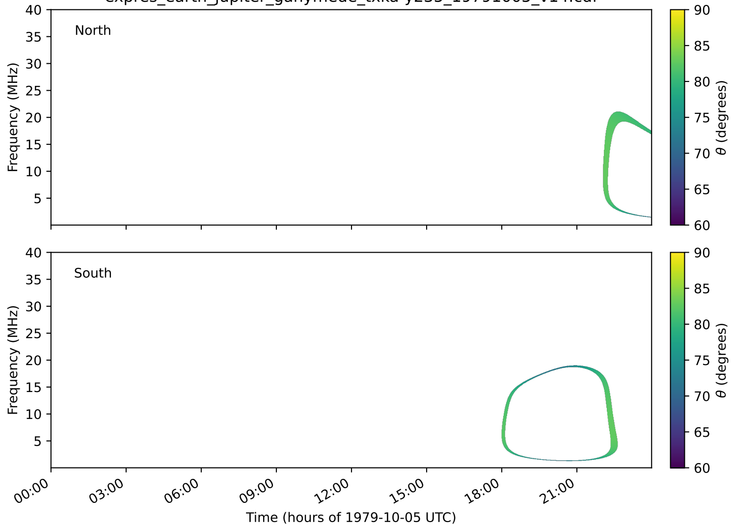
expres_earth_jupiter_ganymede_txka-y235_19791005_v14.cdf
