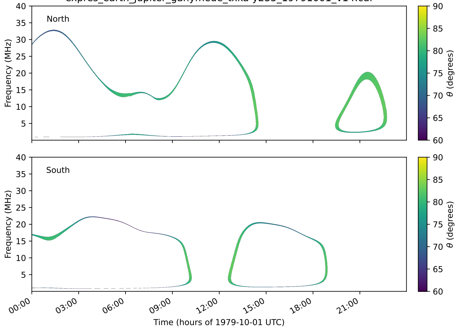
expres_earth_jupiter_ganymede_txka-y235_19791001_v14.cdf
