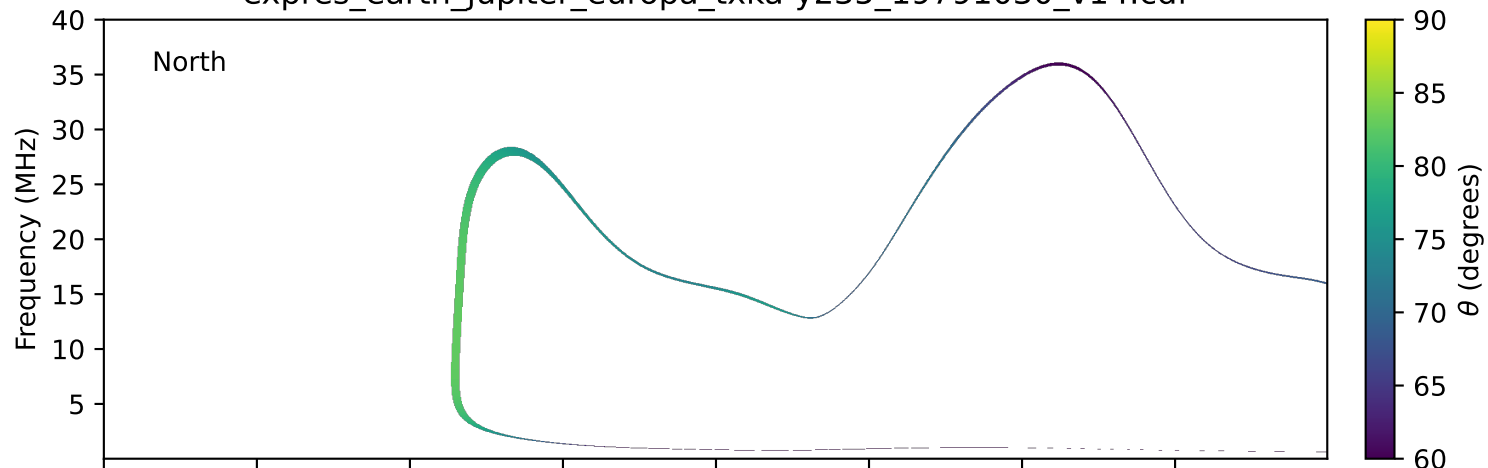
expres_earth_jupiter_europa_txka-y235_19791030_v14.cdf
