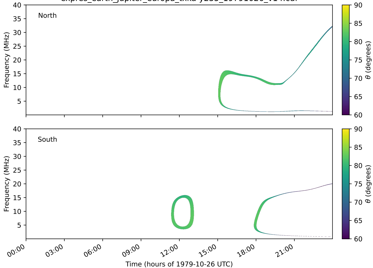
expres_earth_jupiter_europa_txka-y235_19791026_v14.cdf
