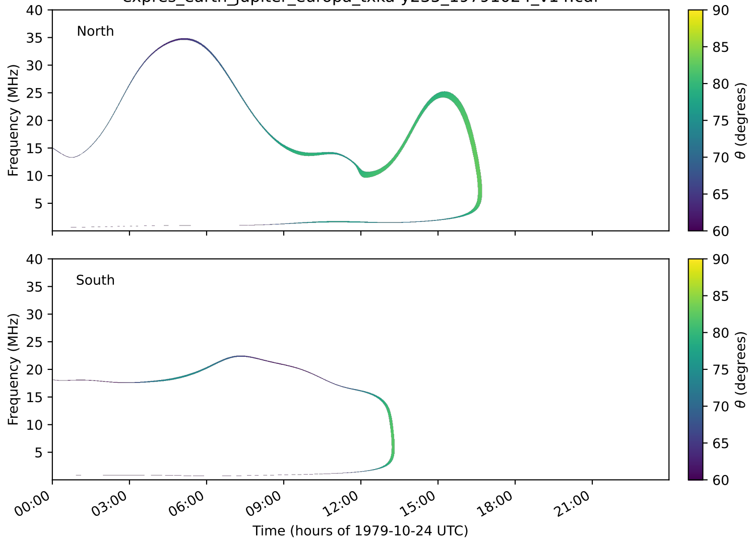
expres_earth_jupiter_europa_txka-y235_19791024_v14.cdf
