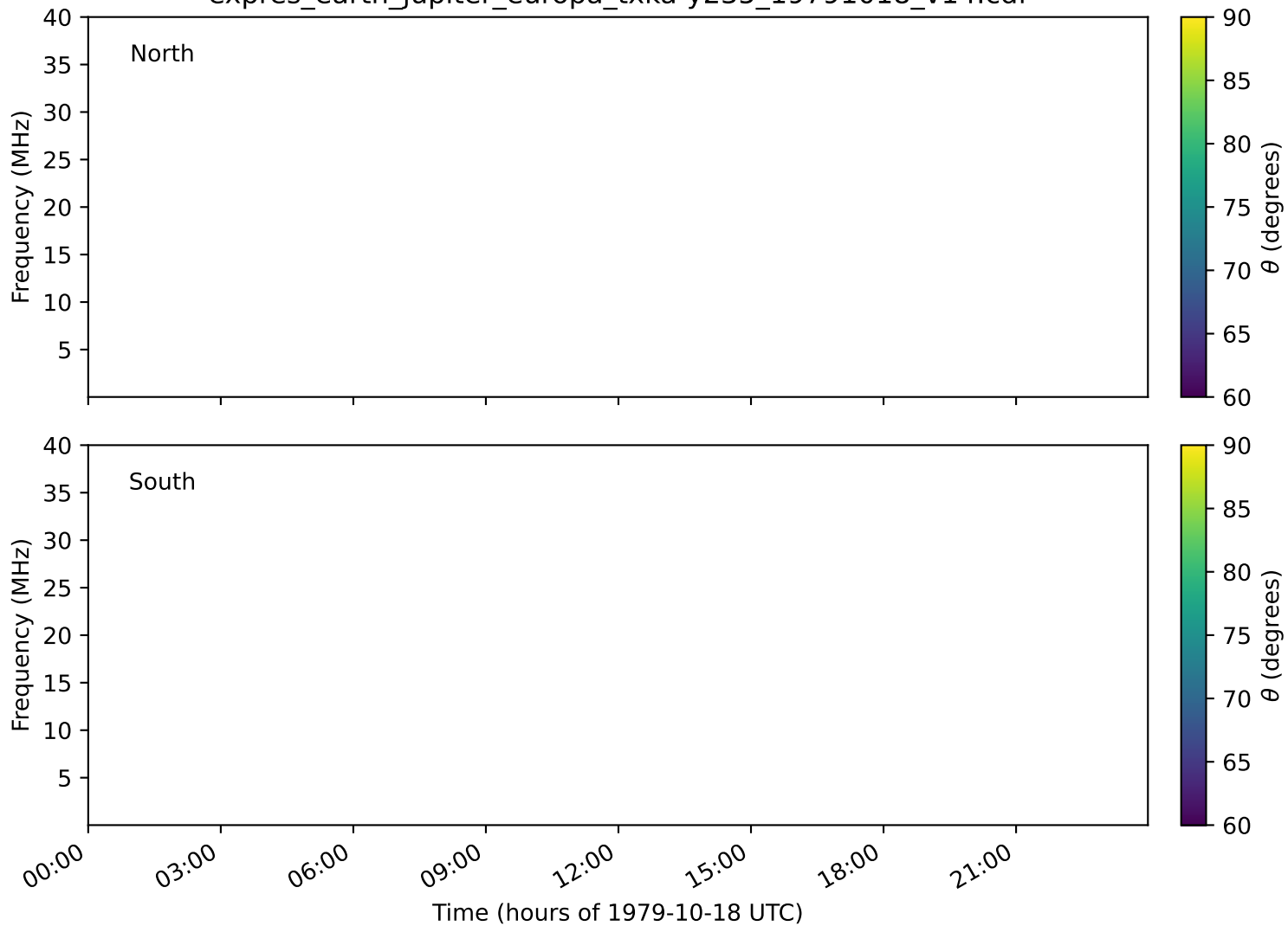
expres_earth_jupiter_europa_txka-y235_19791018_v14.cdf
