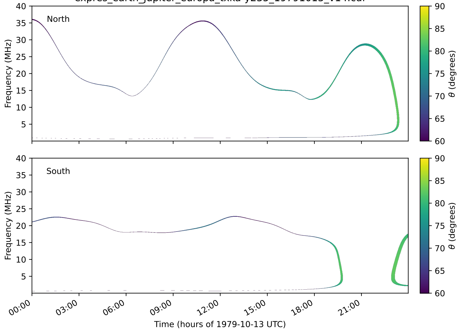
expres_earth_jupiter_europa_txka-y235_19791013_v14.cdf
