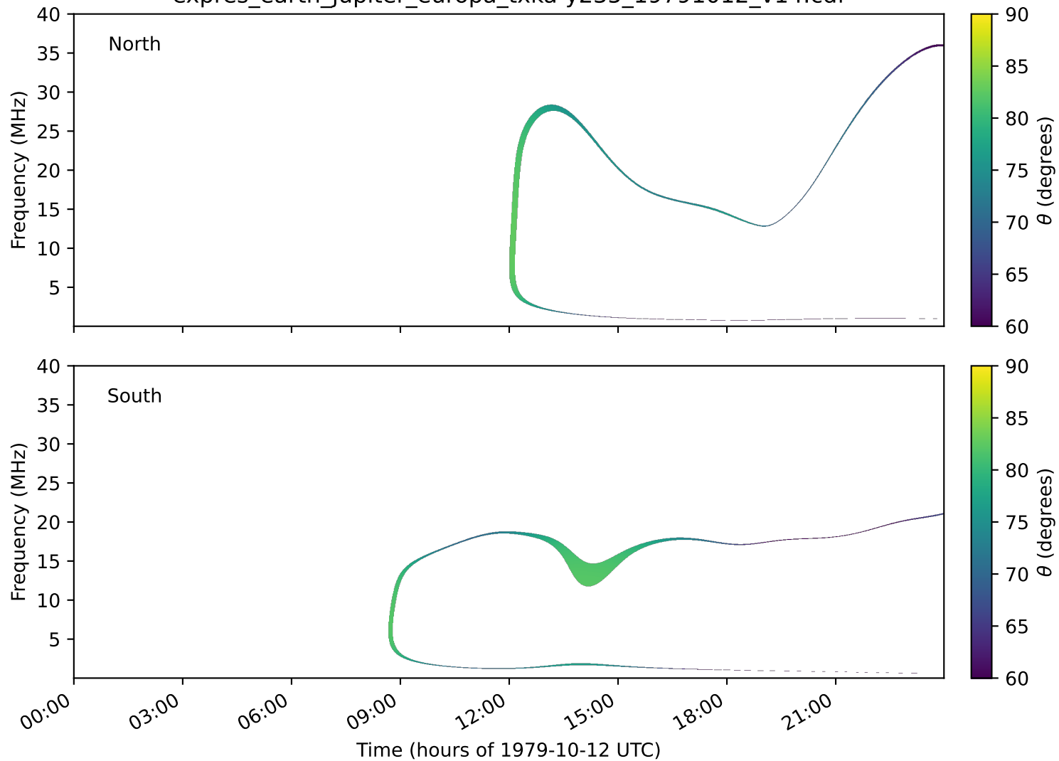
expres_earth_jupiter_europa_txka-y235_19791012_v14.cdf
