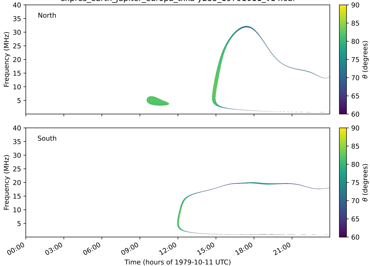
expres_earth_jupiter_europa_txka-y235_19791011_v14.cdf
