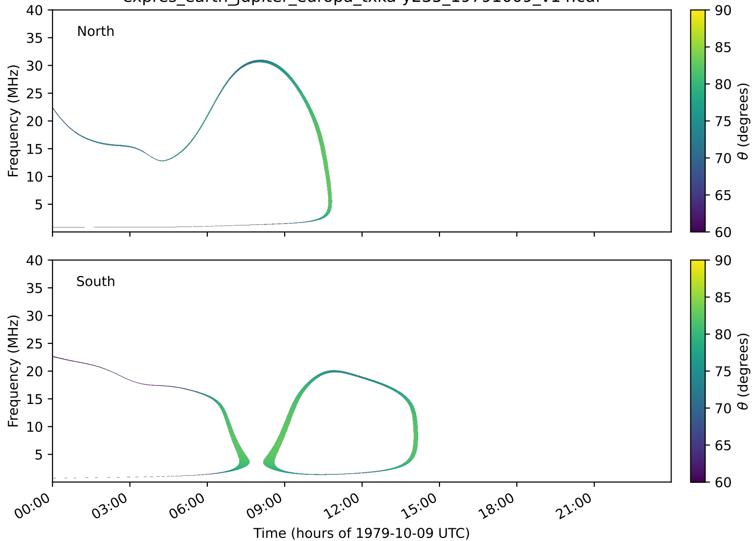
expres_earth_jupiter_europa_txka-y235_19791009_v14.cdf
