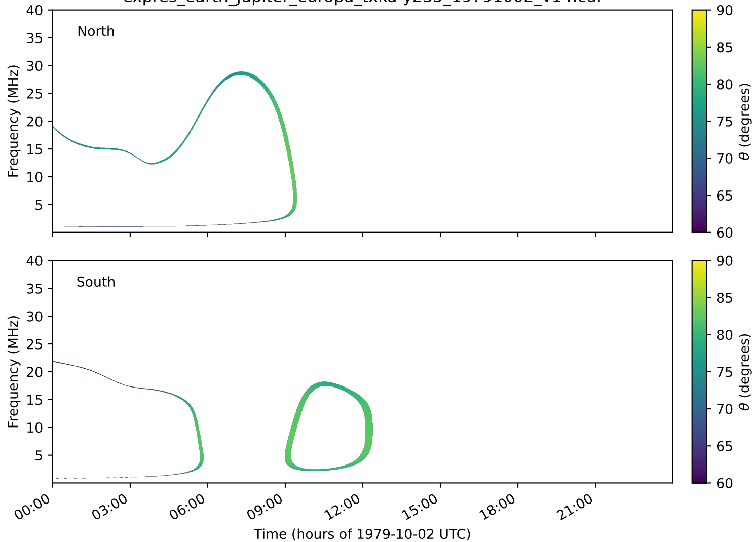
expres_earth_jupiter_europa_txka-y235_19791002_v14.cdf
