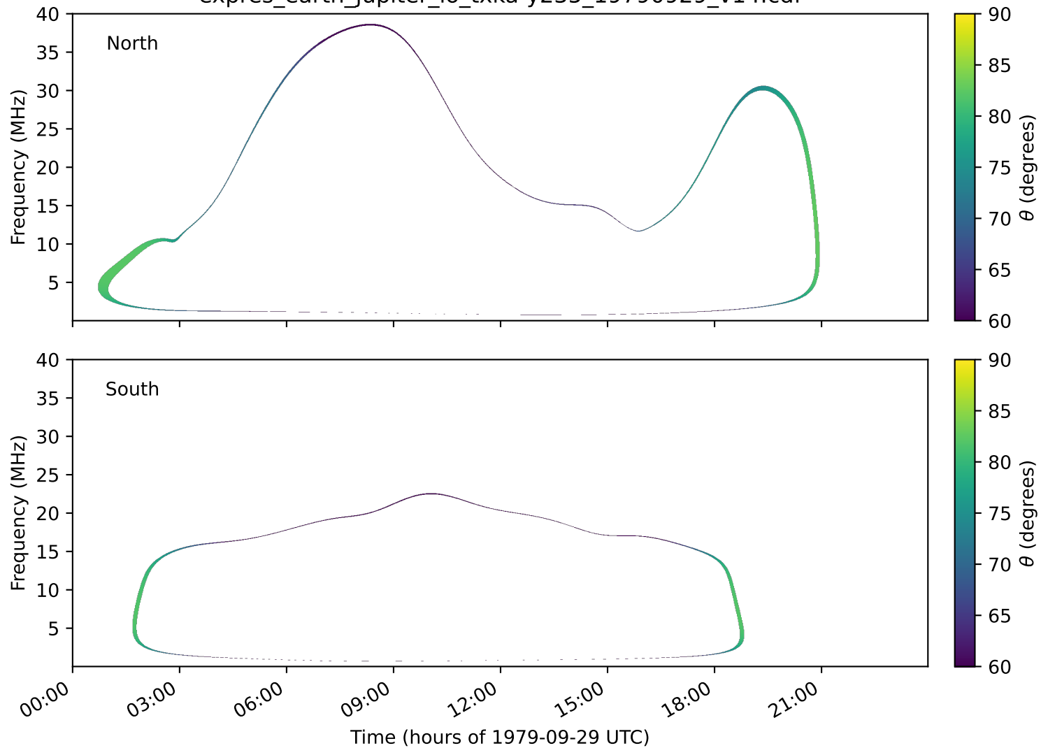
expres_earth_jupiter_io_txka-y235_19790929_v14.cdf
