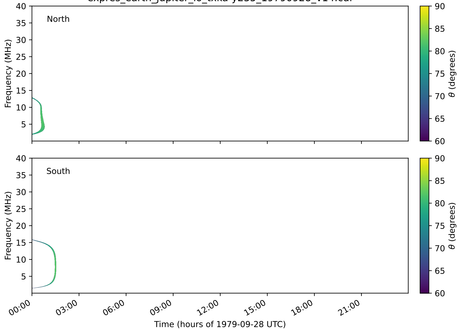
expres_earth_jupiter_io_txka-y235_19790928_v14.cdf
