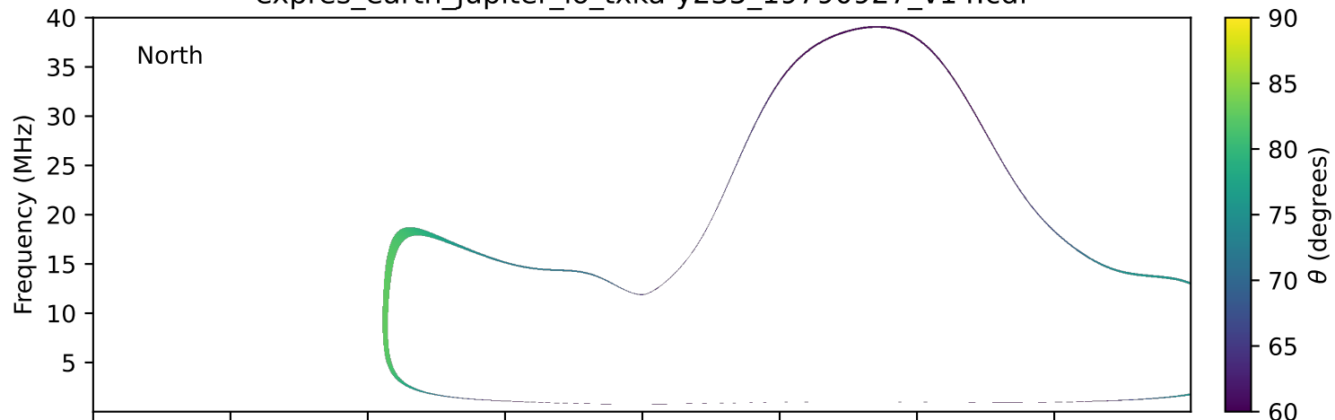
expres_earth_jupiter_io_txka-y235_19790927_v14.cdf
