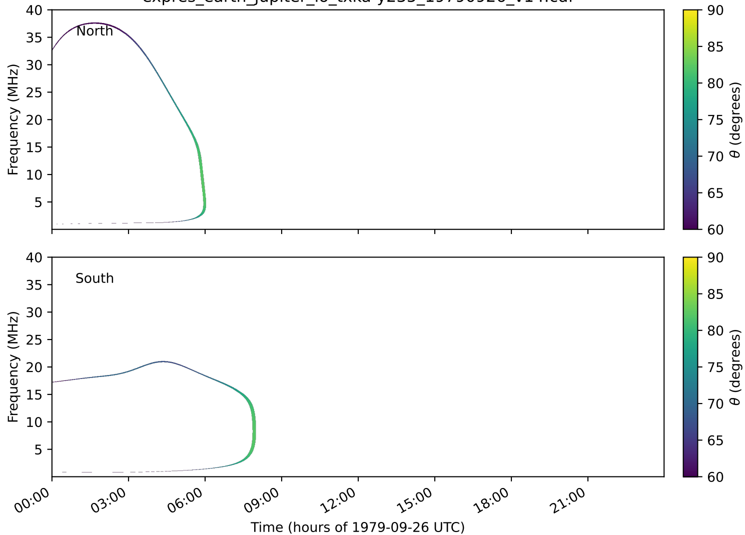
expres_earth_jupiter_io_txka-y235_19790926_v14.cdf
