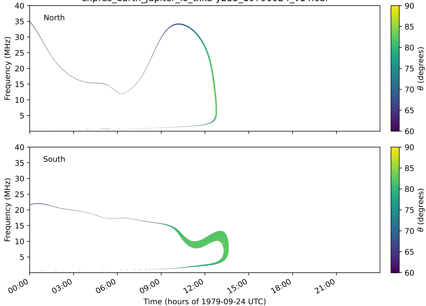
expres_earth_jupiter_io_txka-y235_19790924_v14.cdf
