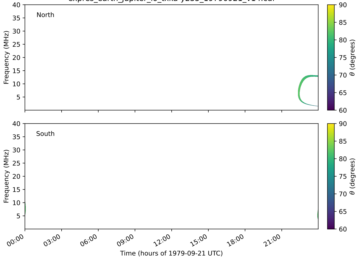
expres_earth_jupiter_io_txka-y235_19790921_v14.cdf
