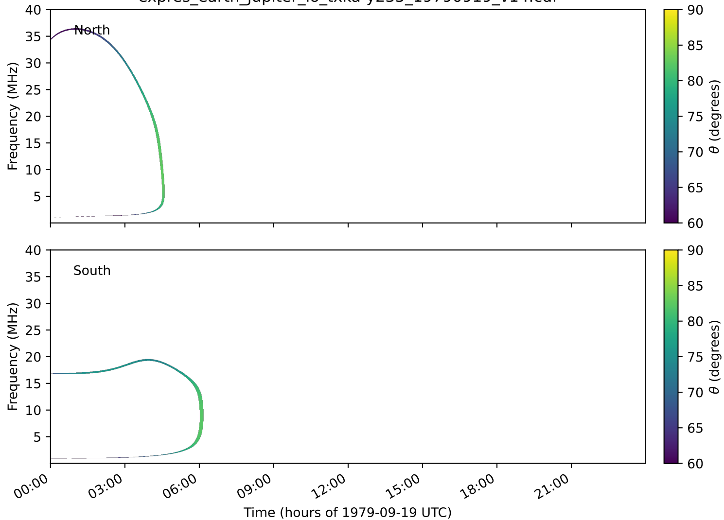
expres_earth_jupiter_io_txka-y235_19790919_v14.cdf
