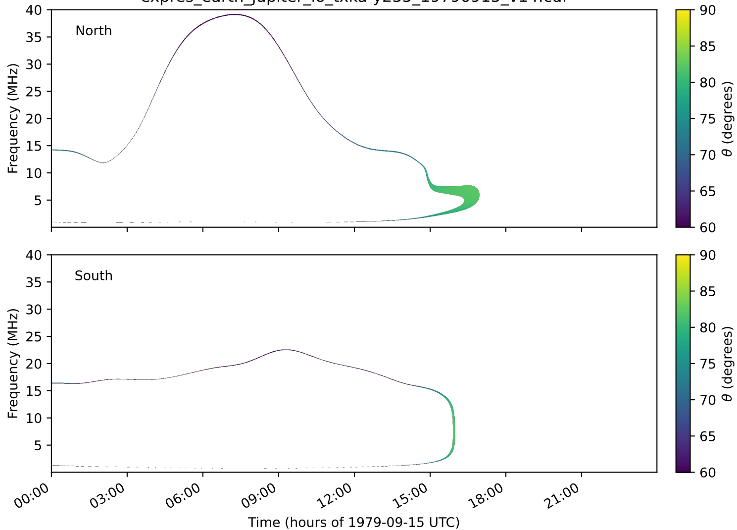
expres_earth_jupiter_io_txka-y235_19790915_v14.cdf
