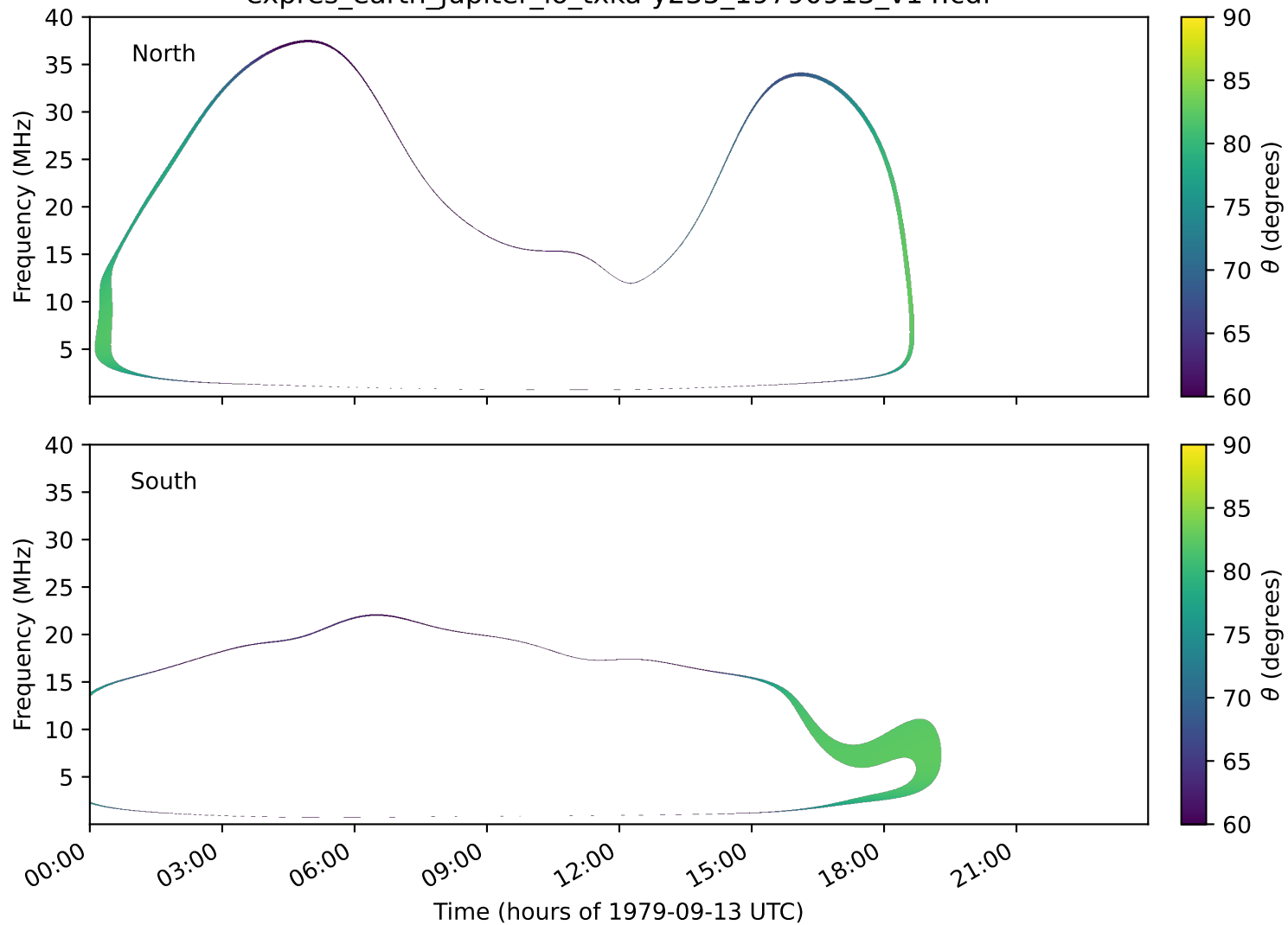
expres_earth_jupiter_io_txka-y235_19790913_v14.cdf
