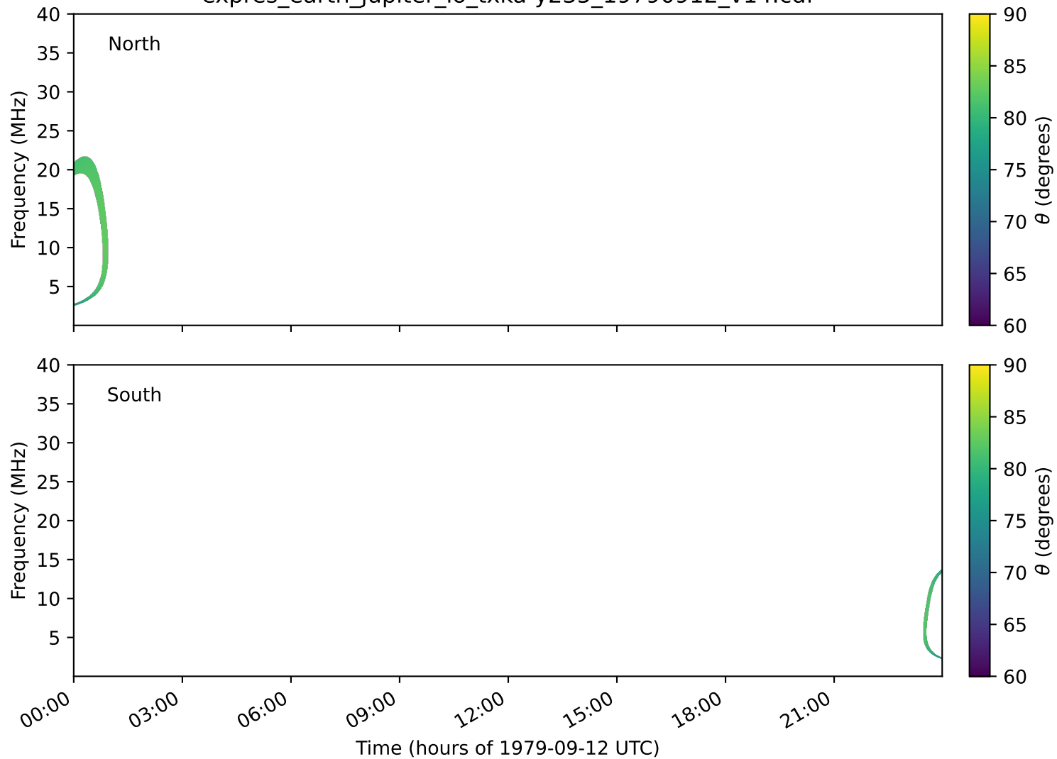
expres_earth_jupiter_io_txka-y235_19790912_v14.cdf
