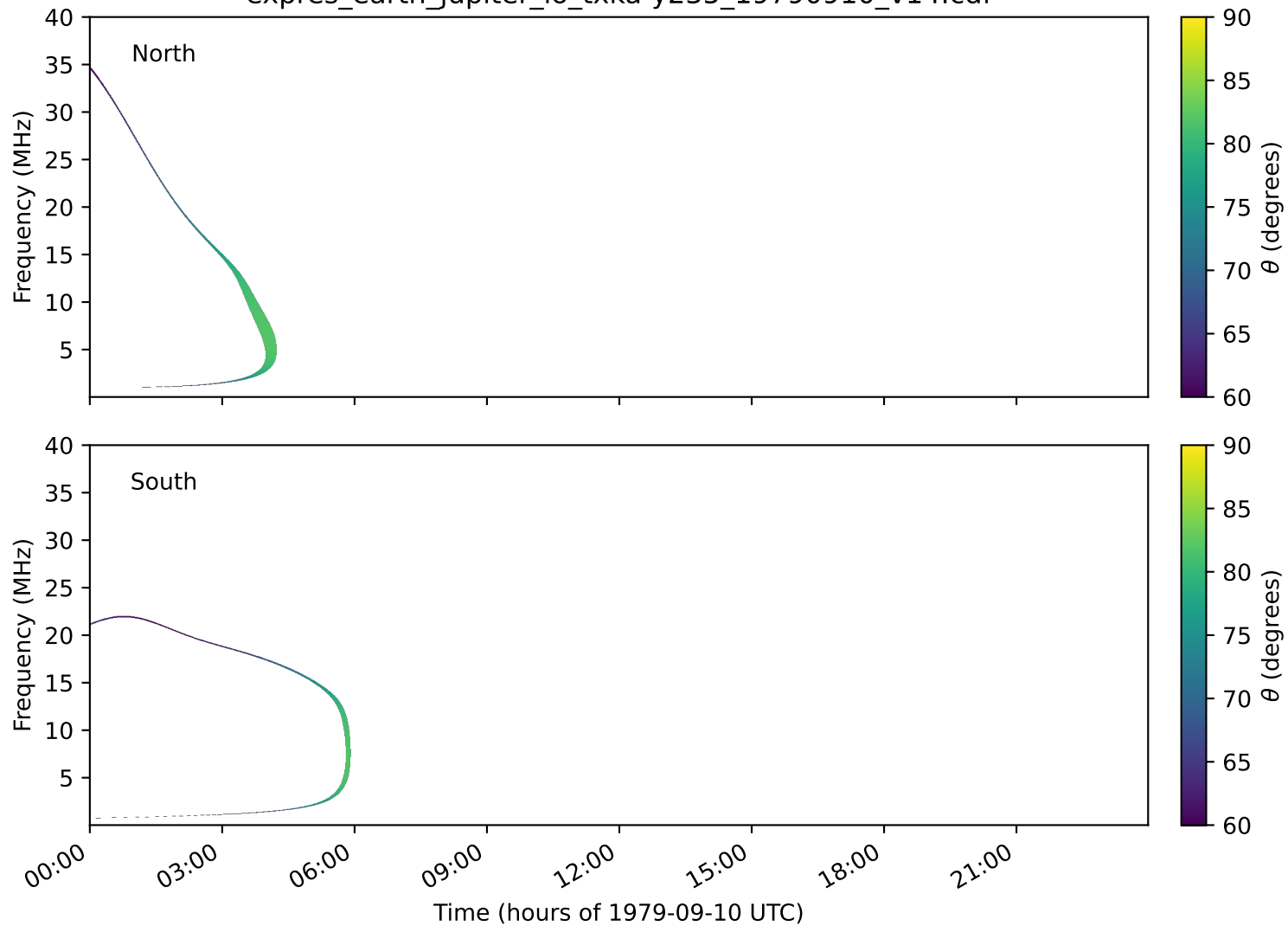
expres_earth_jupiter_io_txka-y235_19790910_v14.cdf
