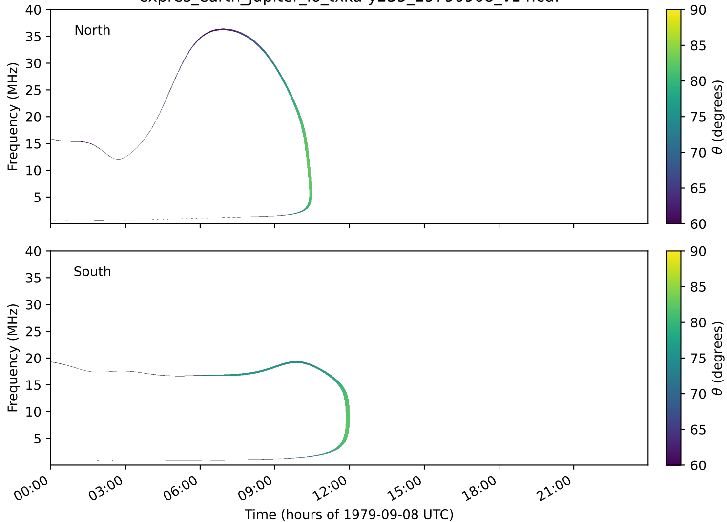
expres_earth_jupiter_io_txka-y235_19790908_v14.cdf
