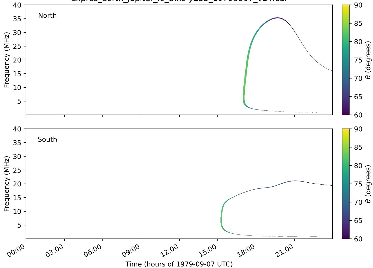
expres_earth_jupiter_io_txka-y235_19790907_v14.cdf
