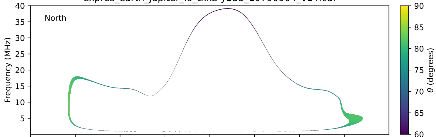
expres_earth_jupiter_io_txka-y235_19790904_v14.cdf
