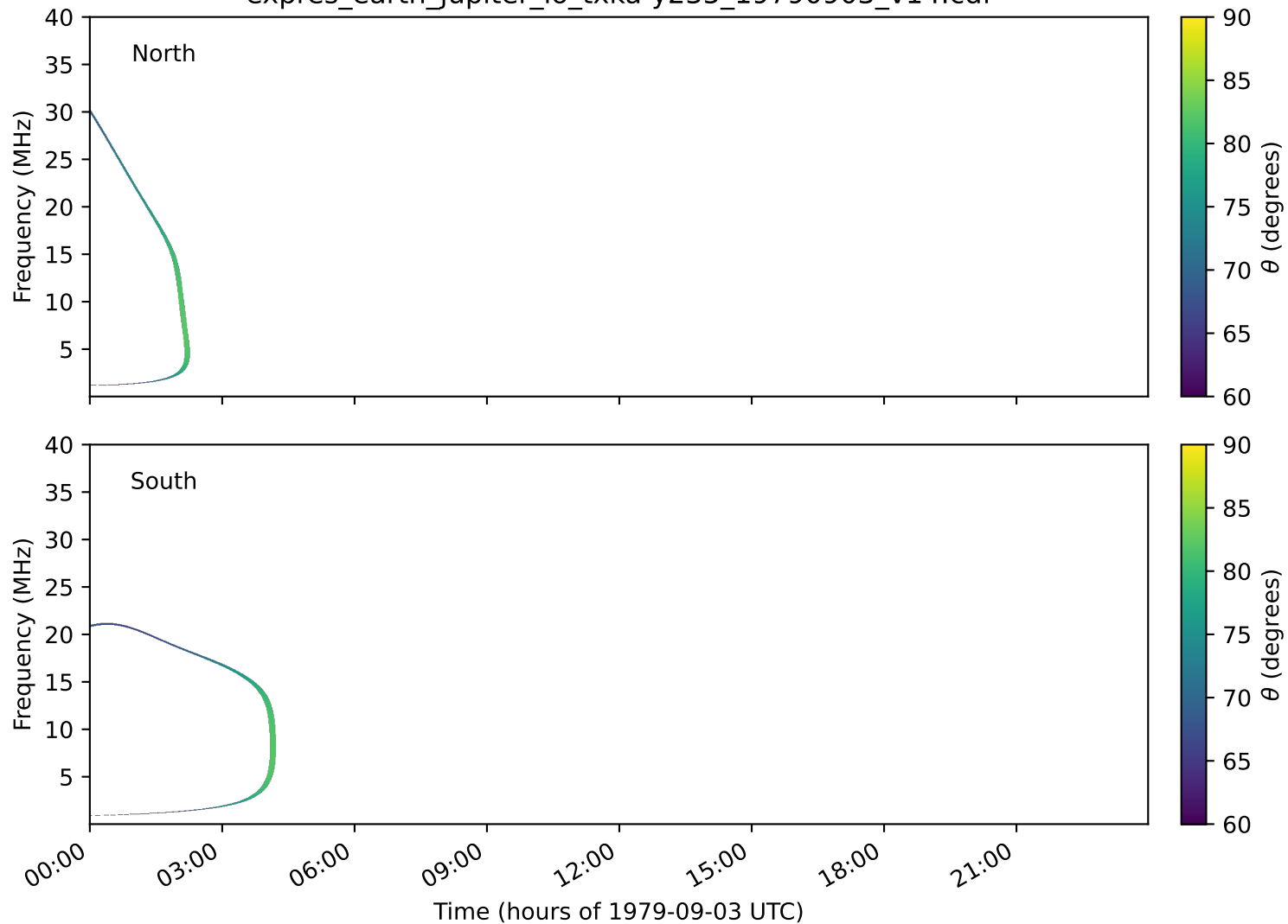
expres_earth_jupiter_io_txka-y235_19790903_v14.cdf
