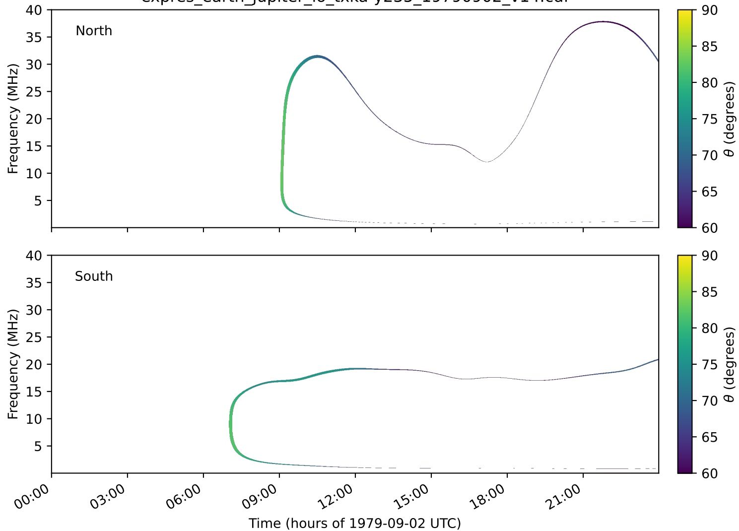
expres_earth_jupiter_io_txka-y235_19790902_v14.cdf
