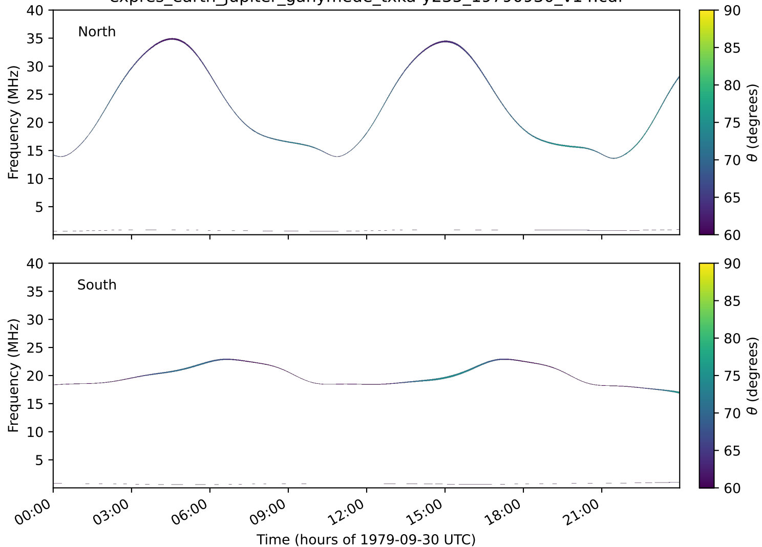
expres_earth_jupiter_ganymede_txka-y235_19790930_v14.cdf
