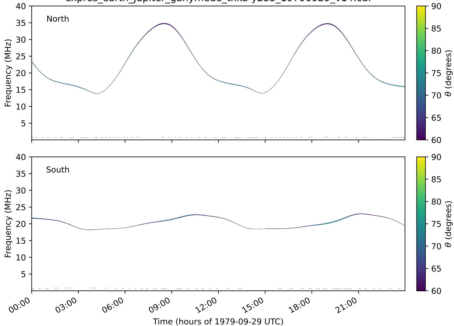
expres_earth_jupiter_ganymede_txka-y235_19790929_v14.cdf
