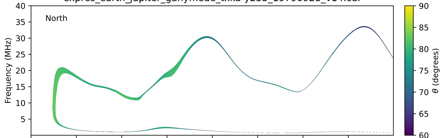
expres_earth_jupiter_ganymede_txka-y235_19790928_v14.cdf
