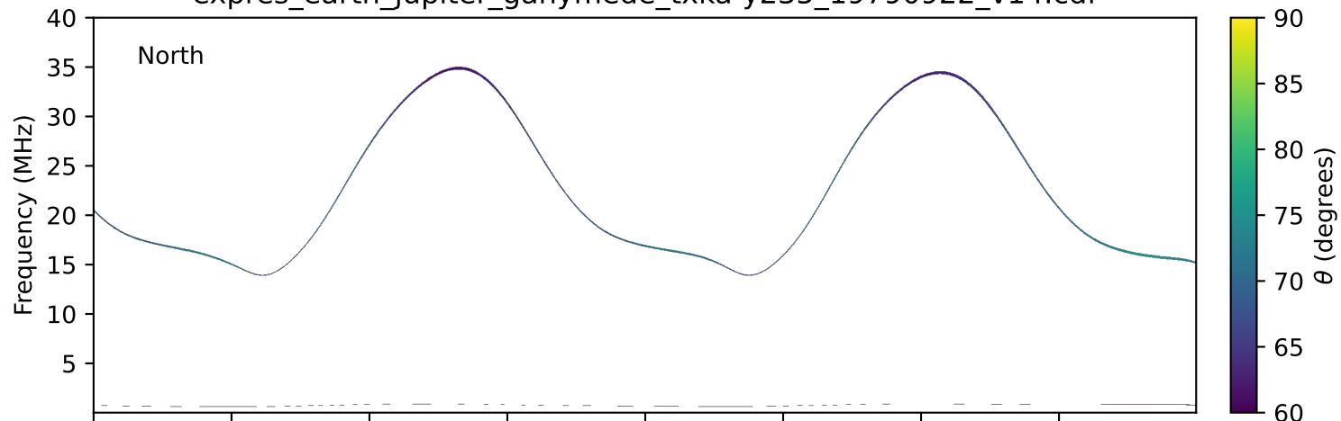
expres_earth_jupiter_ganymede_txka-y235_19790922_v14.cdf
