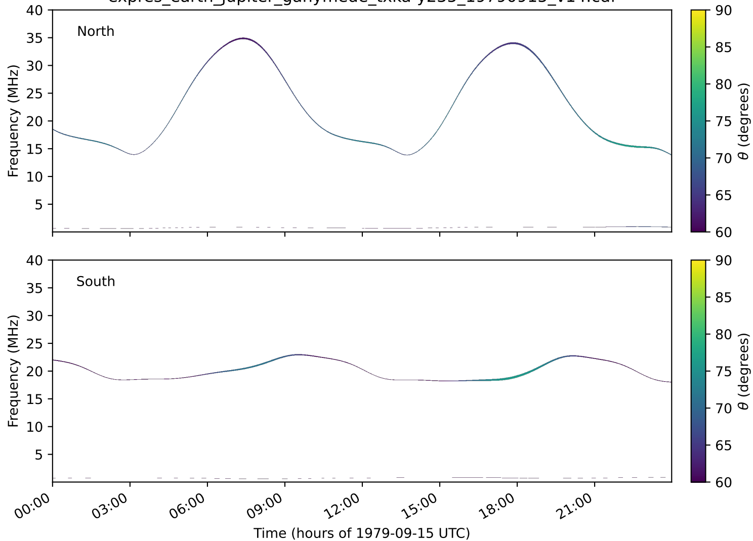
expres_earth_jupiter_ganymede_txka-y235_19790915_v14.cdf
