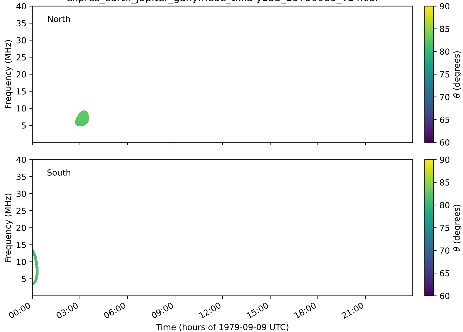
expres_earth_jupiter_ganymede_txka-y235_19790909_v14.cdf
