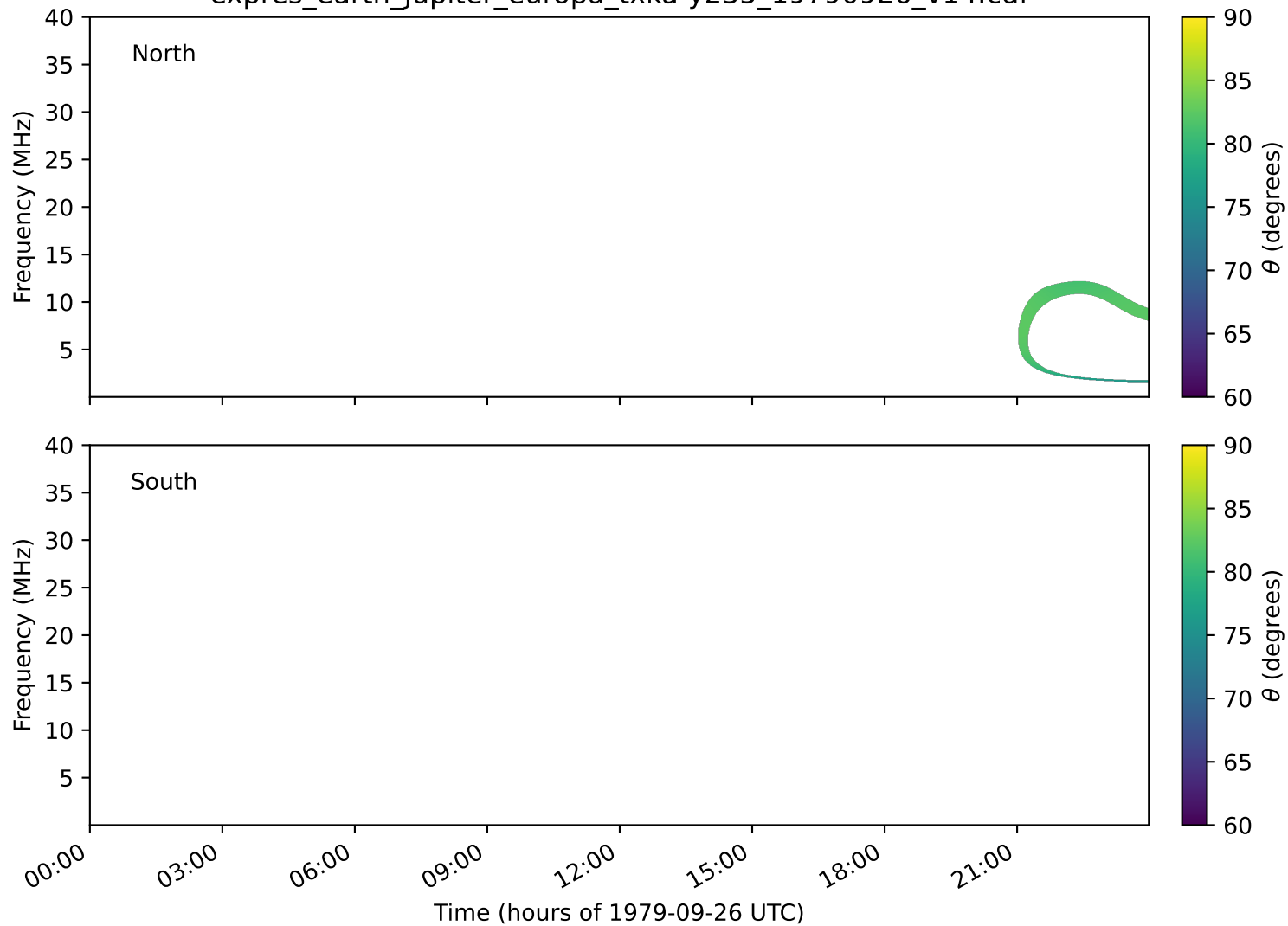
expres_earth_jupiter_europa_txka-y235_19790926_v14.cdf
