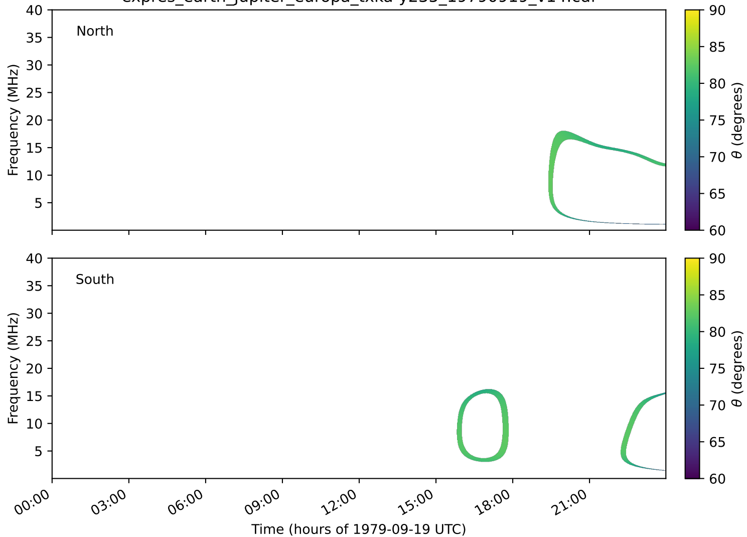
expres_earth_jupiter_europa_txka-y235_19790919_v14.cdf
