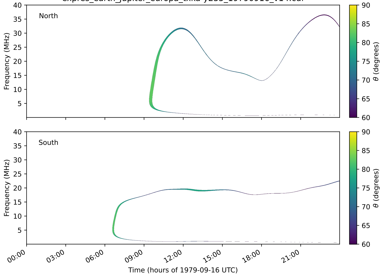
expres_earth_jupiter_europa_txka-y235_19790916_v14.cdf
