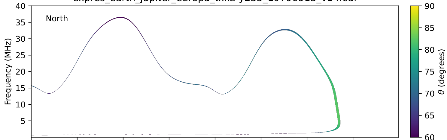
expres_earth_jupiter_europa_txka-y235_19790913_v14.cdf
