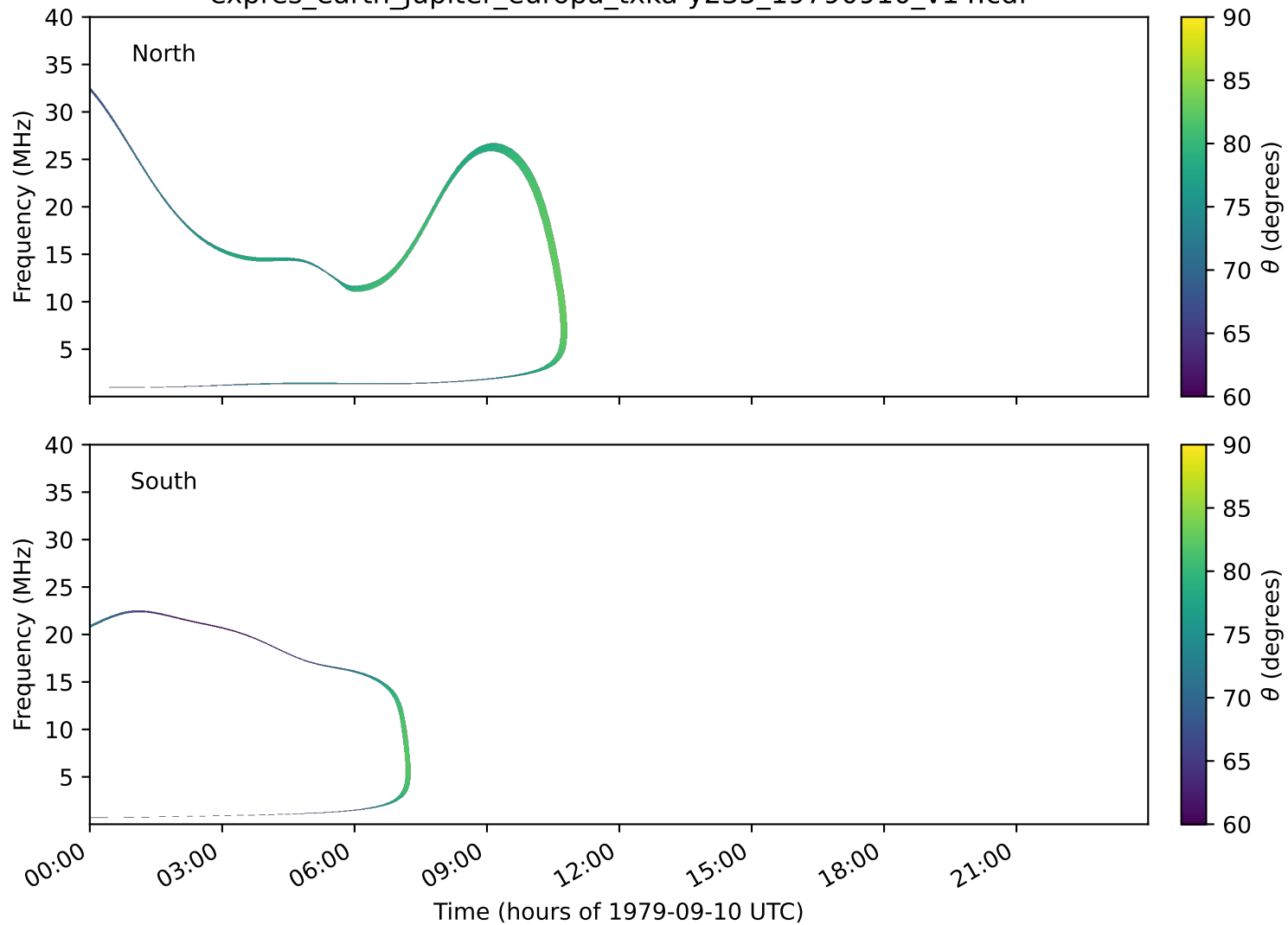
expres_earth_jupiter_europa_txka-y235_19790910_v14.cdf
