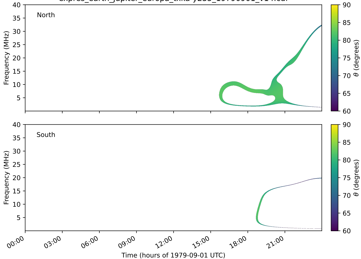
expres_earth_jupiter_europa_txka-y235_19790901_v14.cdf
