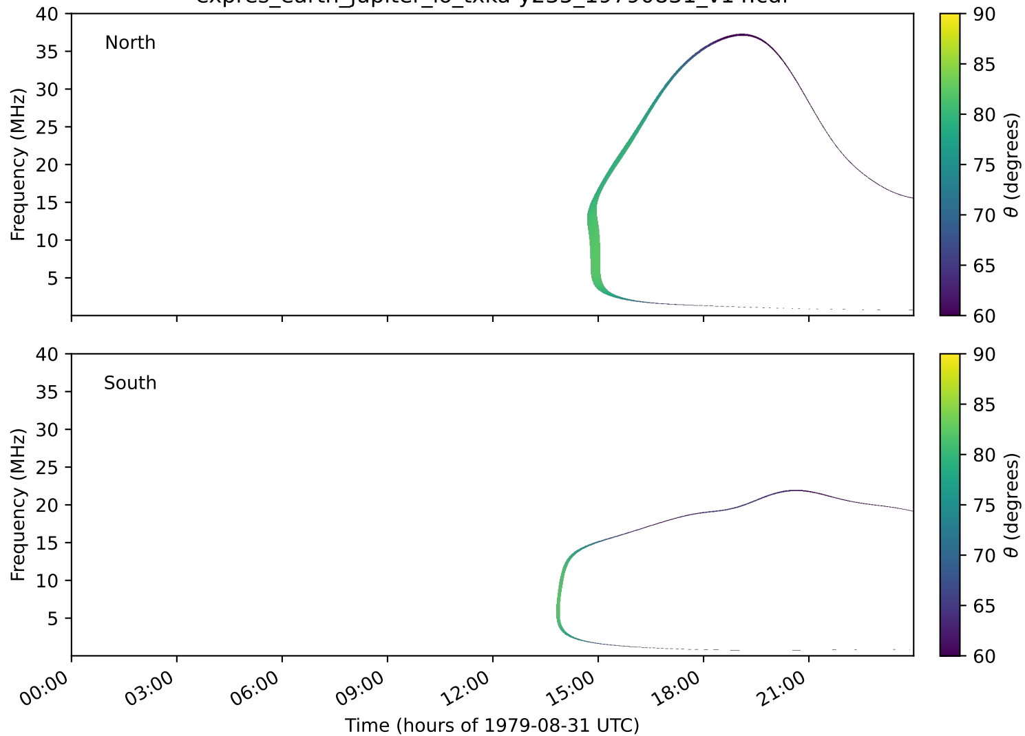
expres_earth_jupiter_io_txka-y235_19790831_v14.cdf
