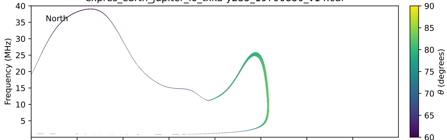
expres_earth_jupiter_io_txka-y235_19790830_v14.cdf
