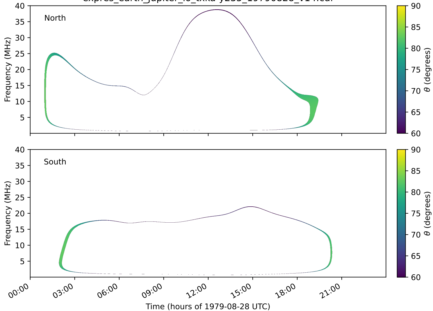
expres_earth_jupiter_io_txka-y235_19790828_v14.cdf
