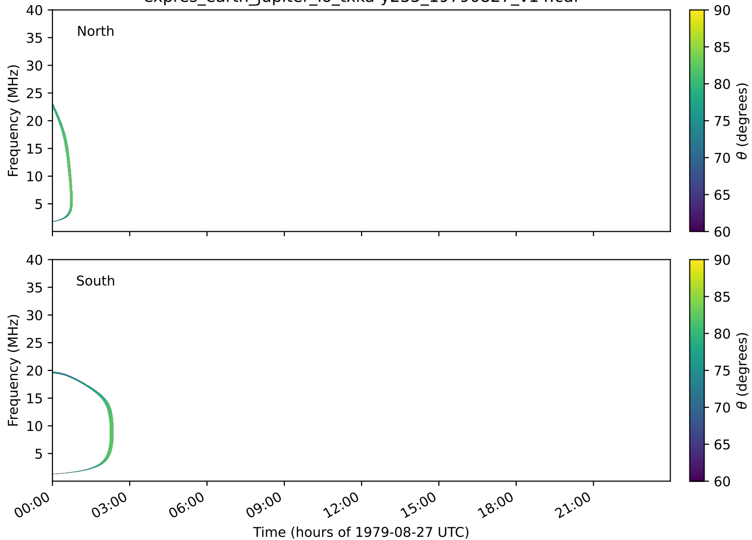
expres_earth_jupiter_io_txka-y235_19790827_v14.cdf
