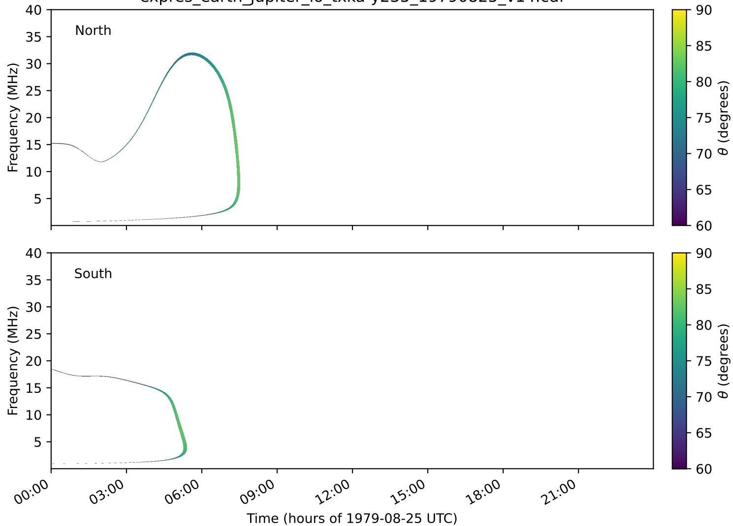
expres_earth_jupiter_io_txka-y235_19790825_v14.cdf
