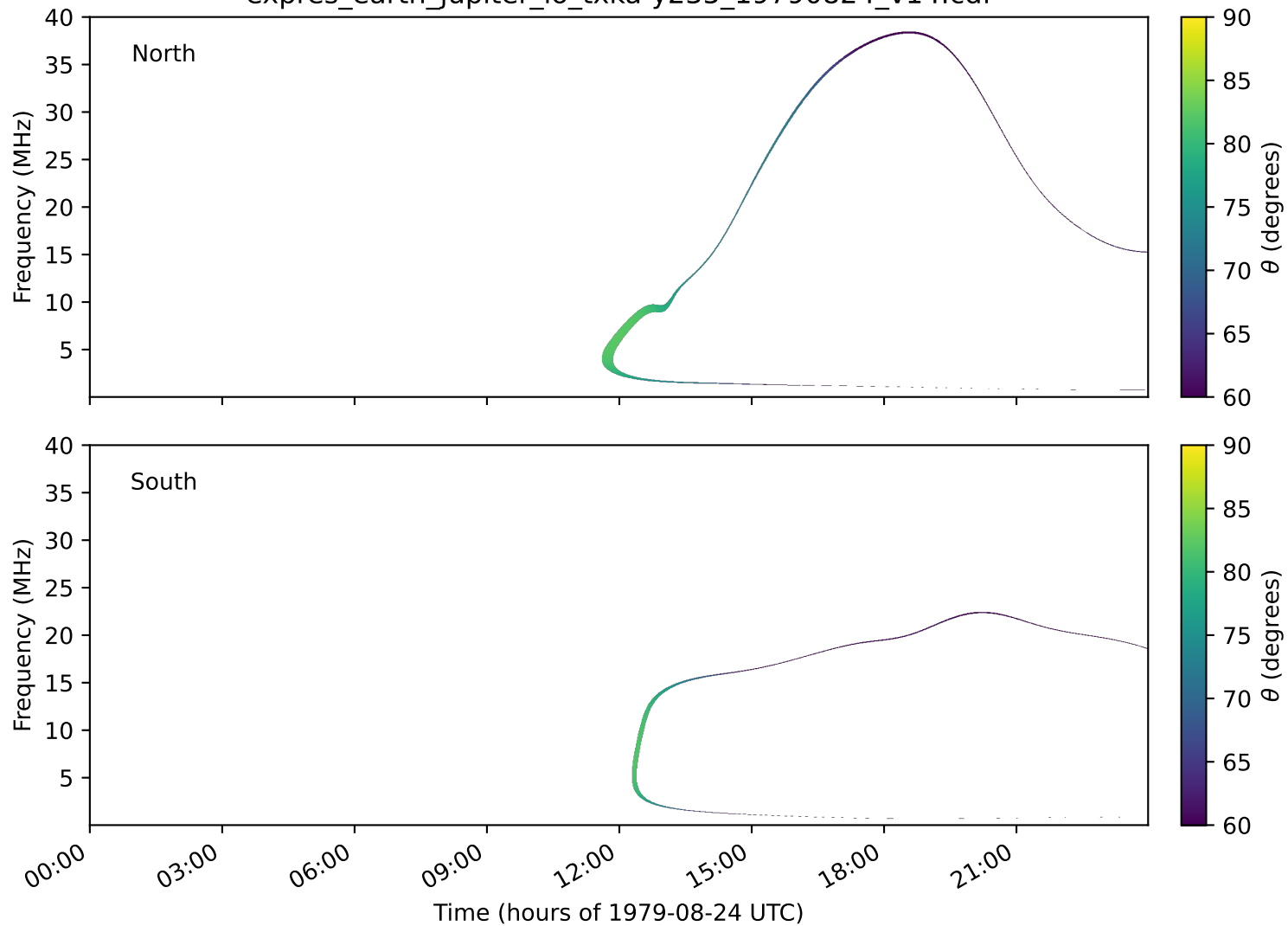
expres_earth_jupiter_io_txka-y235_19790824_v14.cdf
