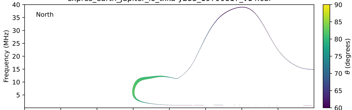
expres_earth_jupiter_io_txka-y235_19790817_v14.cdf
