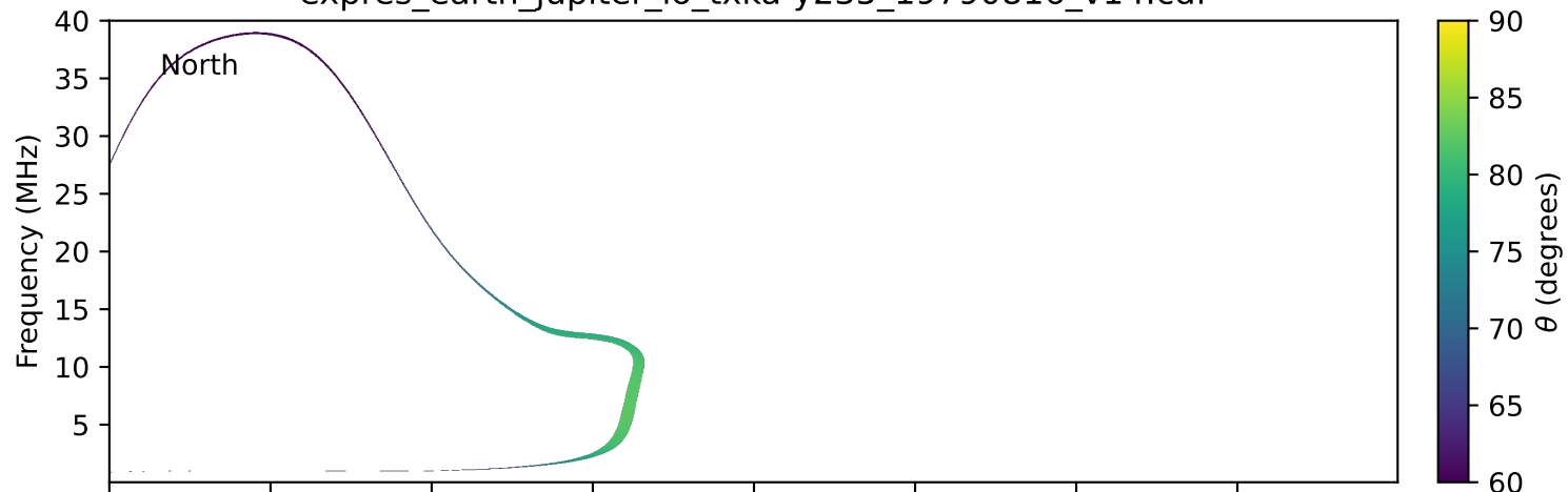
expres_earth_jupiter_io_txka-y235_19790816_v14.cdf
